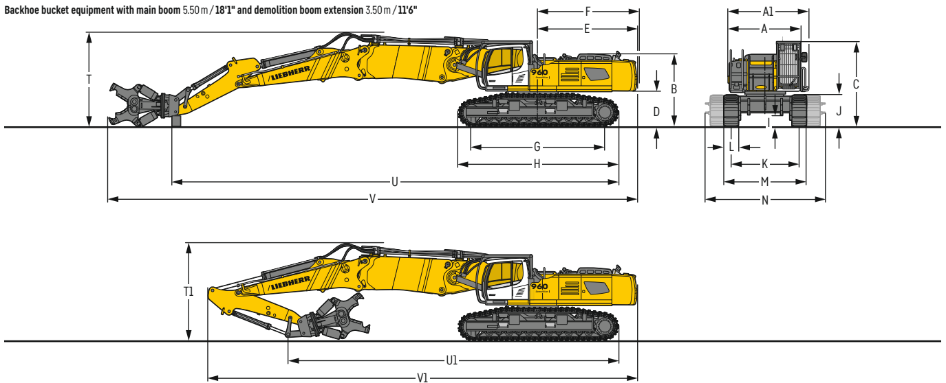
Backhoe bucket equipment with main boom 5.50 m / 18'1" and demolition boom extension 3.50 m / 11'6"
