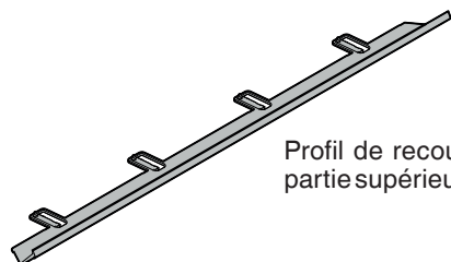
Caches
