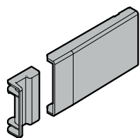
Caches
