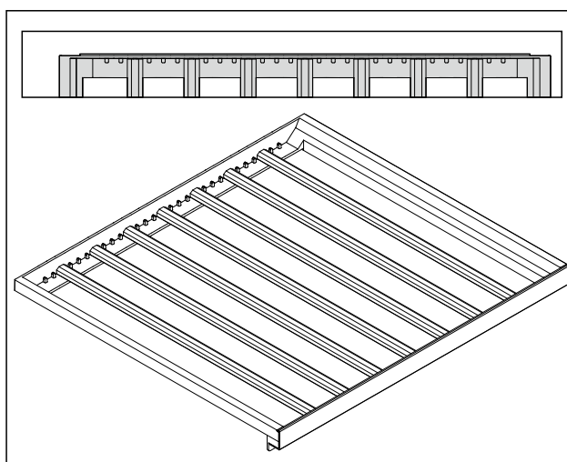
Fig. 103 Arrangement of the bars for maximum number of bottles.
