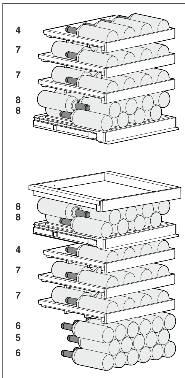
Fig. 14 Total of 85 bottles (for 0.75 l Bordeaux bottles)
