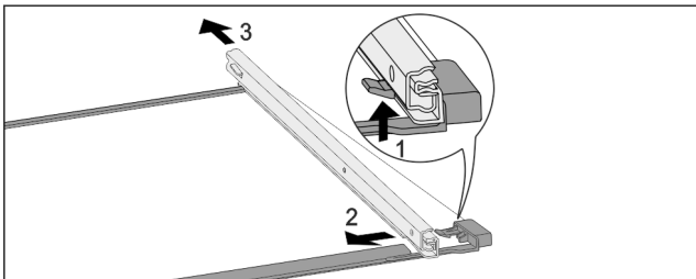
Fig. 115 Glass shelf with rails
