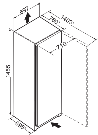
FNc 6625 FNa 6635 FNa 6625 FNd 6625 [mm]
