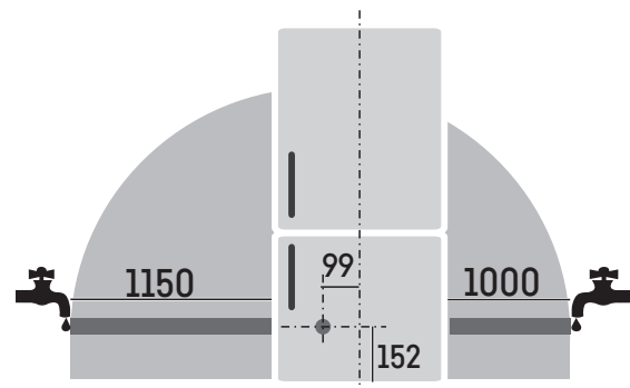
CBNste 8872 CBNstb 579i CNSfc 574i [mm]
