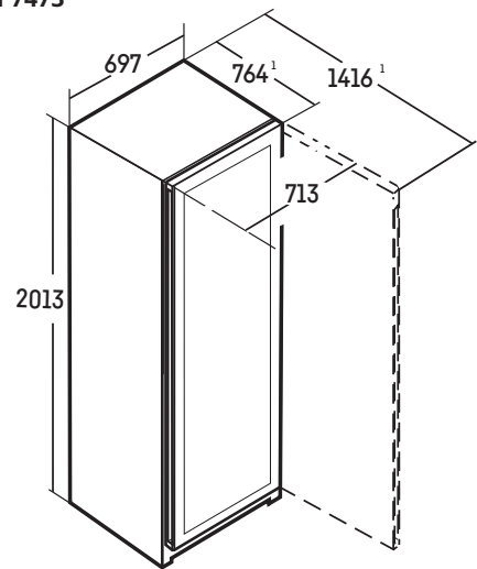
WPgbi 7483 WPgbi 7472 WPgbi 7473 [mm]
