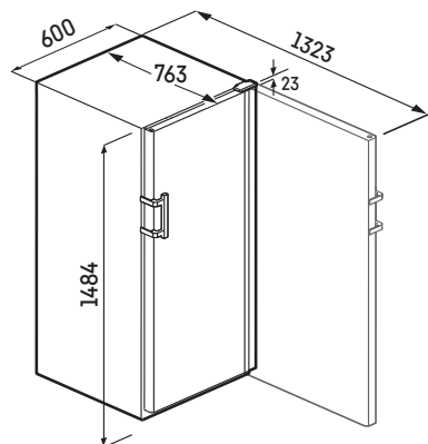
WPbli 4601 WSbli 4601 [mm]
