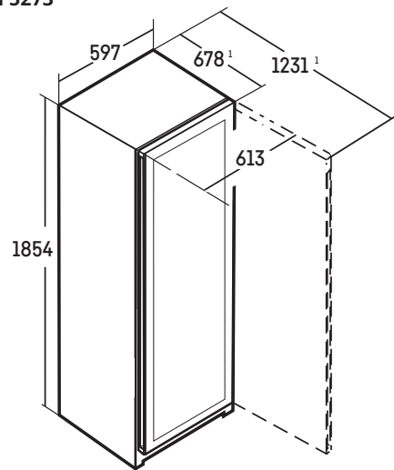
WPgbi 5283 WPgbi 5272 WPgbi 5273 [mm]
