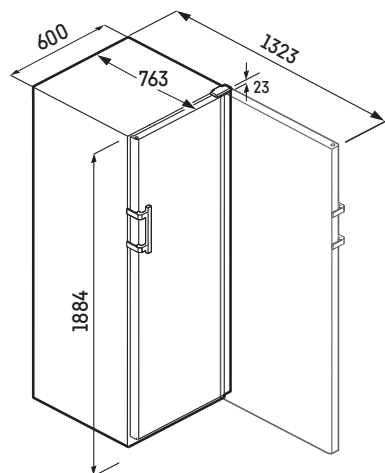
WSbli 5231 WPbli 5231 [mm]
