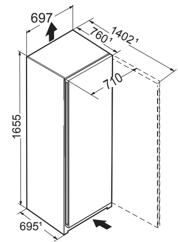
FNc 7026 FNd 7026 [mm]
