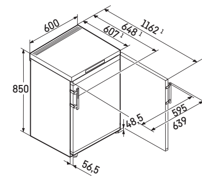
FNdi 1624 FNSddi 1624 Fci 1624 [mm]
