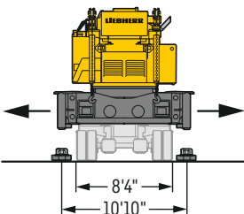
Swinging out the four jack-up cylinders Extension des 4 vérins Jack-Up
