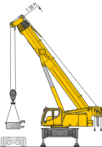
Central ballast assembly (2 x 16,540 lb) Montage du contrepoids central (2 x 16,540 lb)
