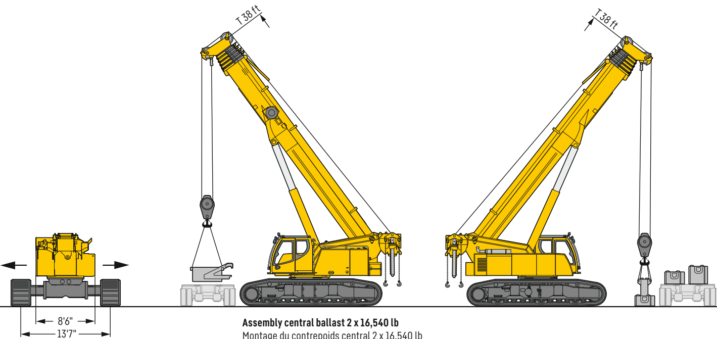
Telescope crawler travel gear out Elargir le train de chenilles
