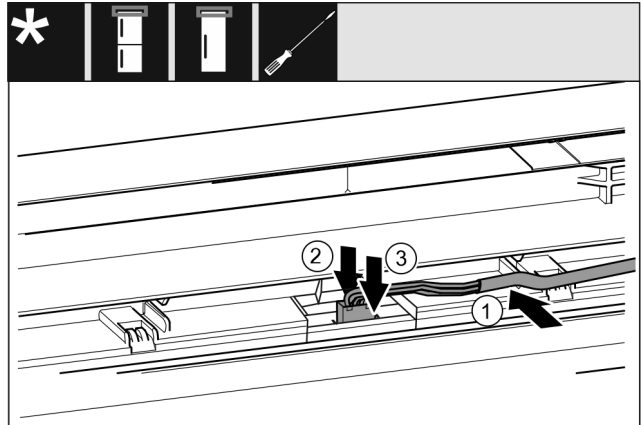
Fig. 40 Fridge/freezer combinations / freezers / refrigerators
