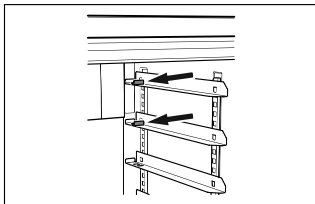
Fig. 60 Stop bracket
