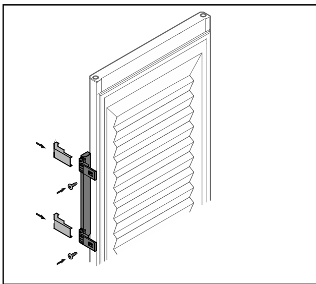
Fig. 24 Insulated door*
