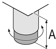
Fig. 8 The adjustable foot can be adjusted from A = 115 \text{ mm} (4 1/2 in) to 175 \text{ mm} (6 7/8 in).
