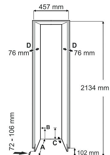
Plinthe continue
