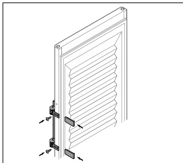
Fig. 34 Insulated door*
