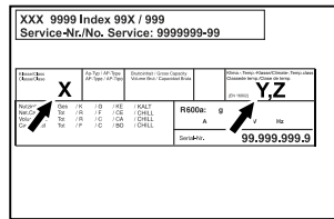
Fig. 1 Type plate
