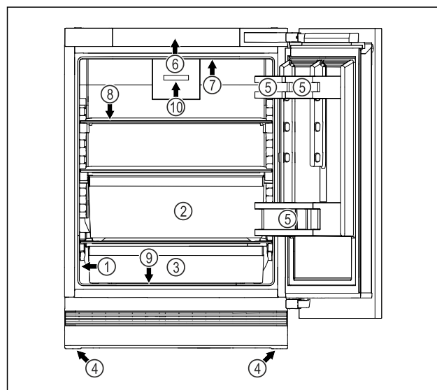
Fig. 1 Exemplary illustration of the front side
