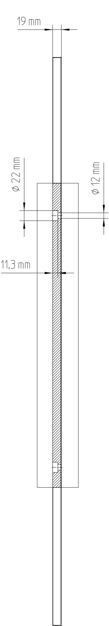
Side view
