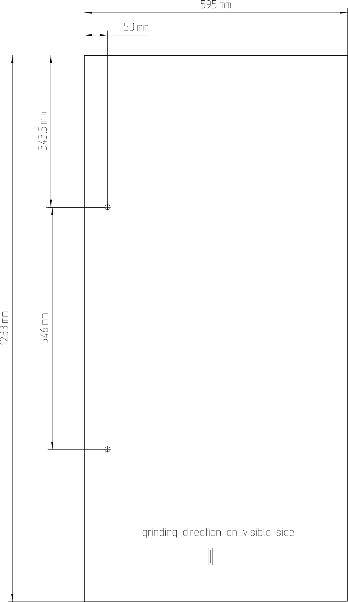
Front view
