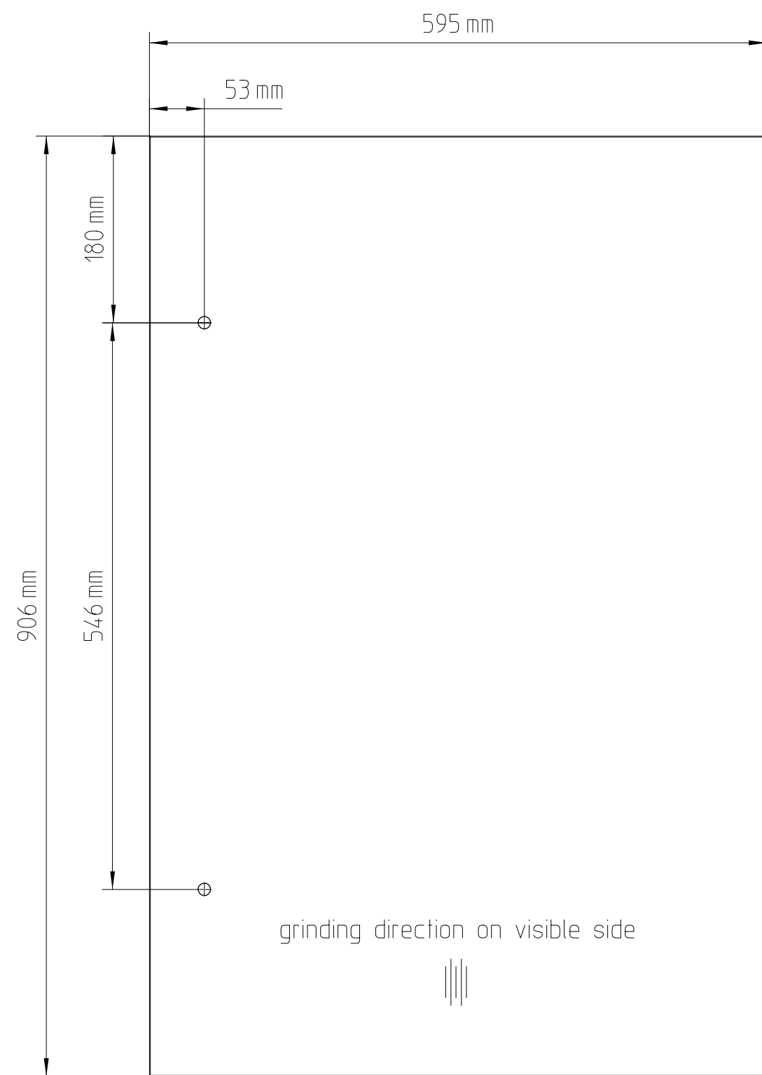
Front view
