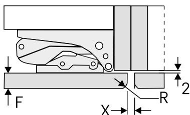
Fig. 67 Joint gap with adjoining unit door
