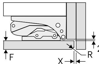
Fig. 66 Joint gap with adjoining furniture side panel
