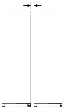
Fig. 11 Side-by-side installation
