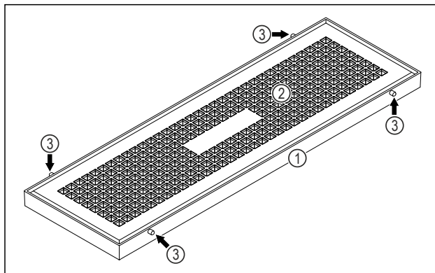
Fig. 102 Example illustration, Water box
