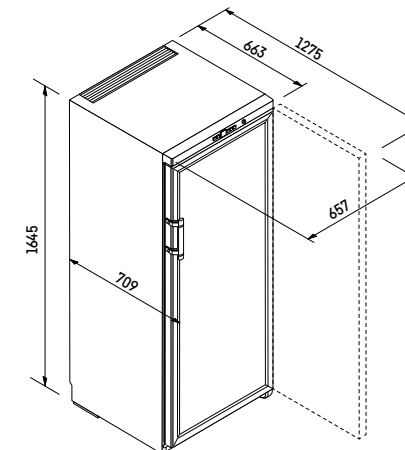
Installation Diagram
