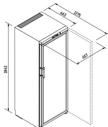
Installation Diagram
