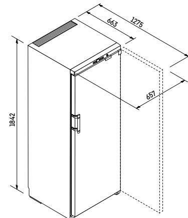
Installation Diagram
