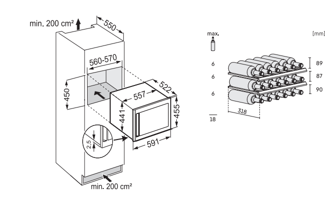
Installation Diagram
