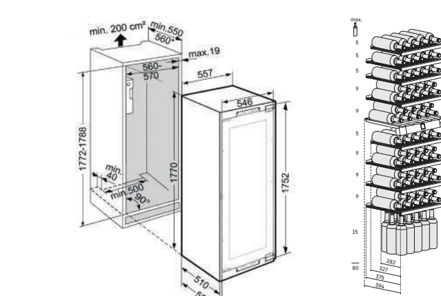
Installation Diagram
