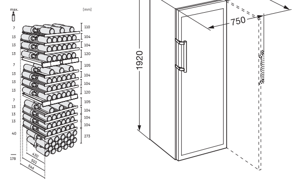
Installation Diagram
