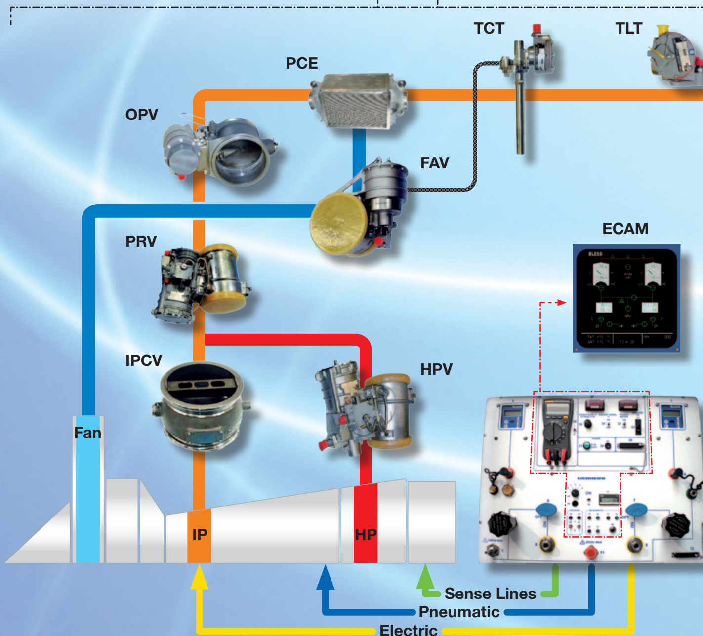
ATA36 Engine Bleed Air System
