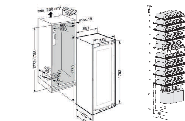
Installation Diagram
