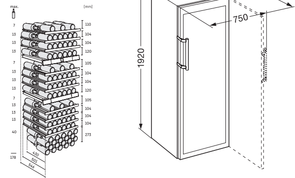
Installation Diagram
