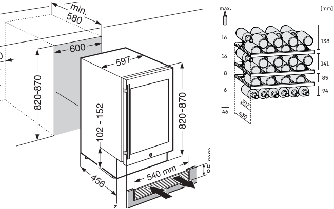
Installation Diagram
