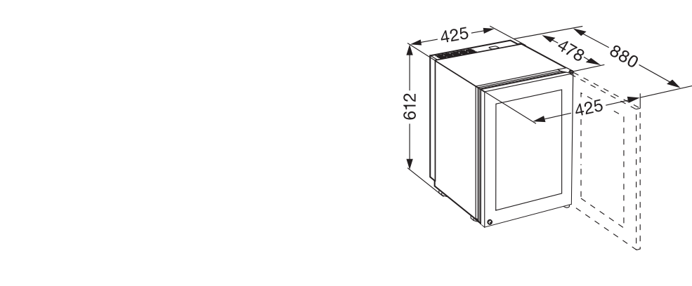
Installation Diagram
