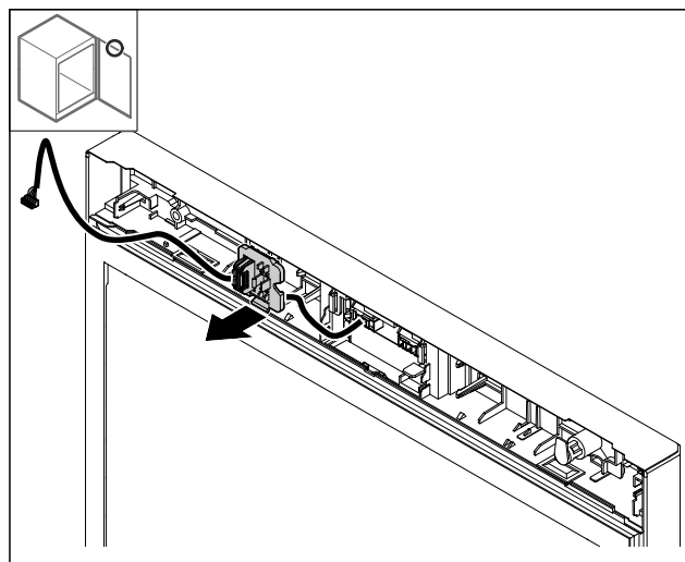
Fig. 30 The installation position for the plug holder can be rotated by 180°.
