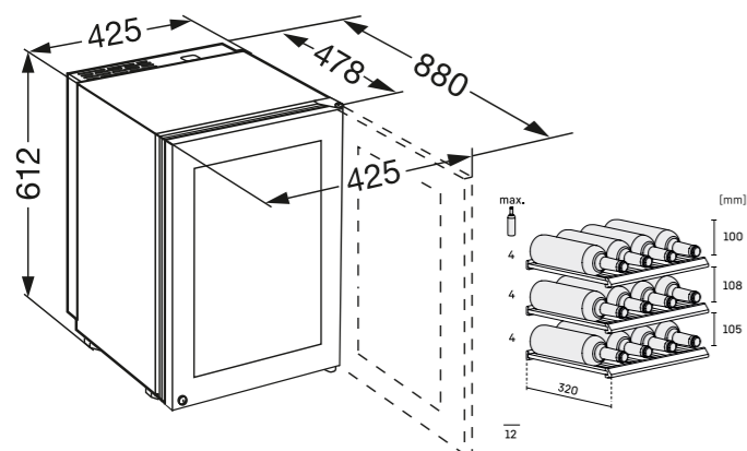
Installation Diagram
