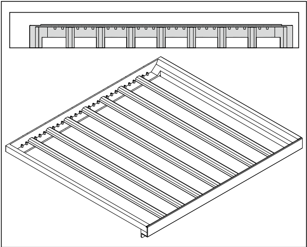
Fig. 73 Arrangement of the bars for maximum number of bottles.
