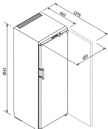
Installation Diagram
