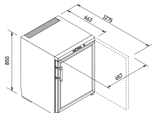
Installation Diagram
