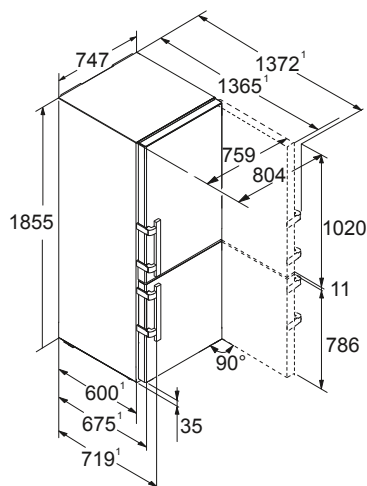
Installation Diagram
