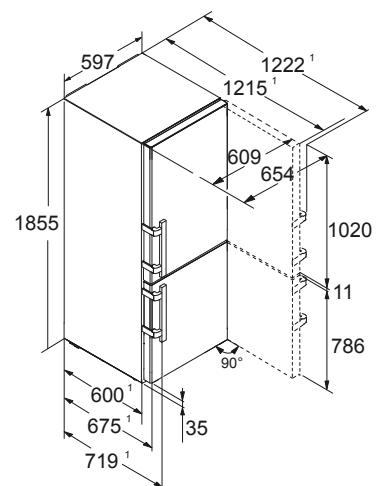
Installation Diagram
