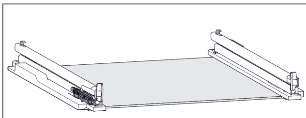
Fig. 120 Damping mechanism
